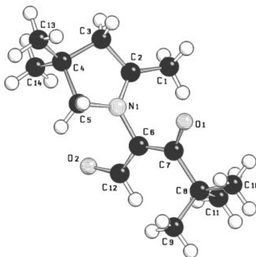
Figure 1. Crystal structure of the azomethine ylide 25b (SCHAKAL drawing, hydrogen atoms omitted; the numbering does not correspond with the correct nomenclature); selected bond lengths [Å] and angles [°]: C2–N 1.292, N–C5 1.467, N–C6 1.445, C2–C3 1.491, C3–C4 1.531, C4–C5 1.541, C6–C7 1.429, C6–C12 1.395; C2–N–C5 112.7, C2–N–C6 126.2, C7–C6–N 116.1, C2–N–C5 112.7, C7–C6–C12 130.5; angle between the planes C5–N–C2 and C7–C6–C12 72.7
